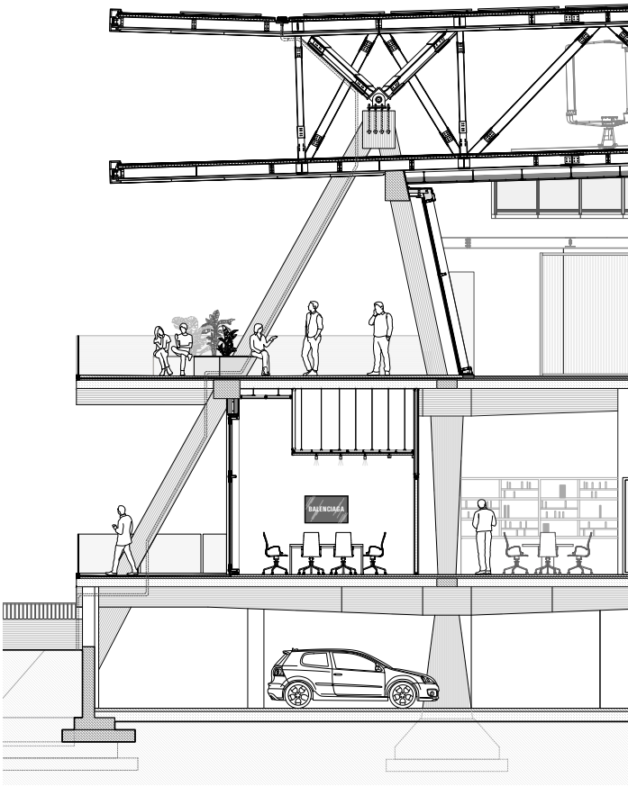
Technological section
