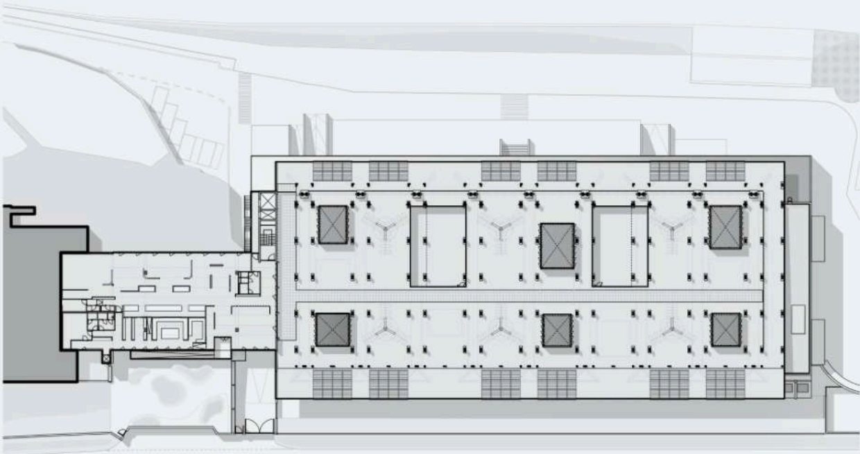
Grundriss 4. Obergeschoss fourth upper level floor plan
